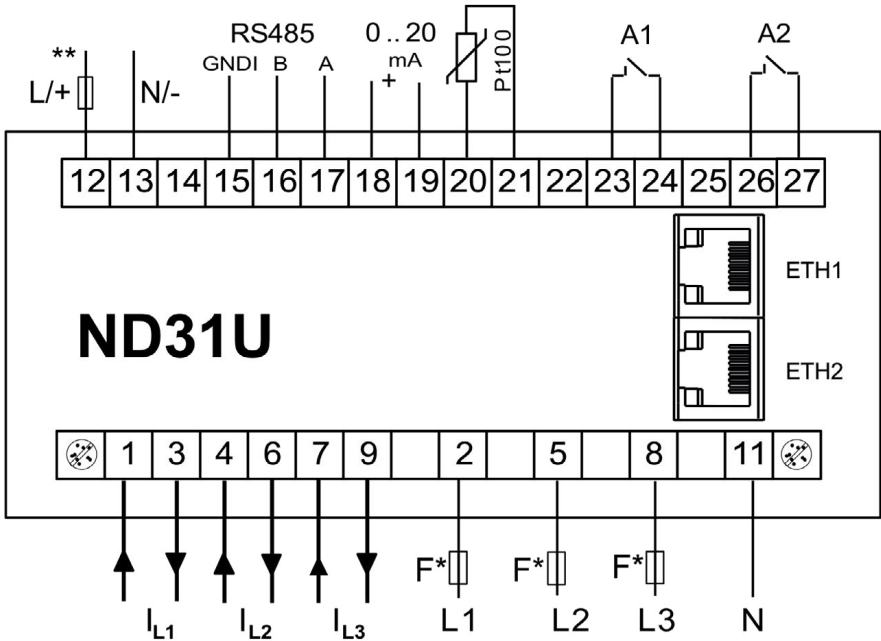
Fig. 4. Meter connections
